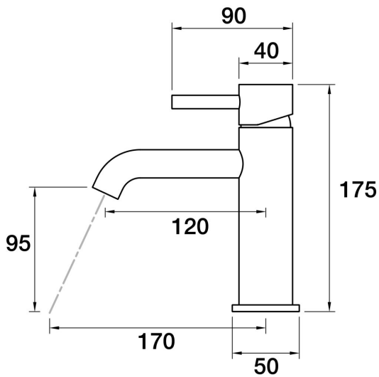
Lugano Hob Basin Mixer A22.011.2.01 - Chrome
