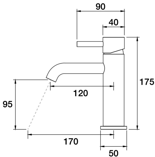
Lugano Hob Basin Mixer A22.011.2.25 - Brushed Nickel
