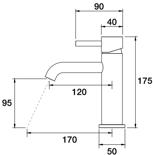
Lugano Hob Basin Mixer A22.011.2.43 - Brass
