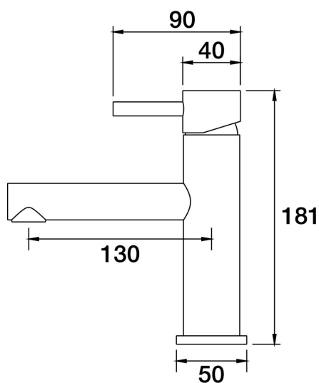
Lugano Hob Basin Mixer Straight A22.011.3.67 - Vintage Brass
