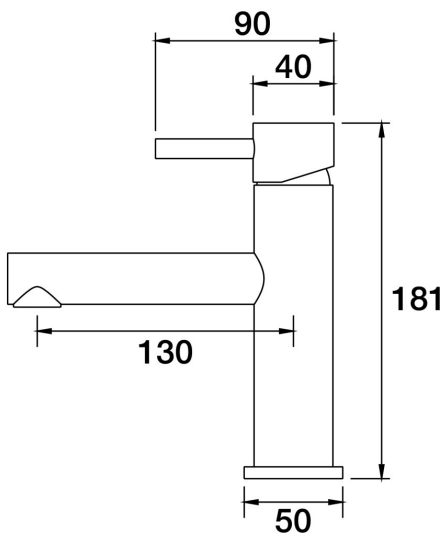
Lugano Hob Basin Mixer Straight A22.011.3.77 - Oud Bronze
