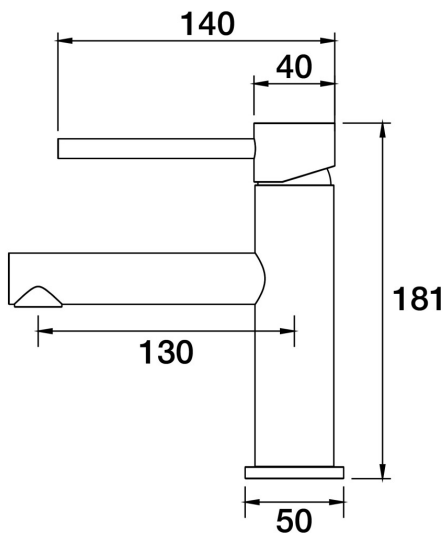
Lugano Hob Basin Mixer Straight DDA Compliant A22.011.4.21 - Brushed Rose Gold
