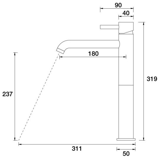
Lugano Hob Basin Tower Mixer A22.012.1.01 - Chrome
