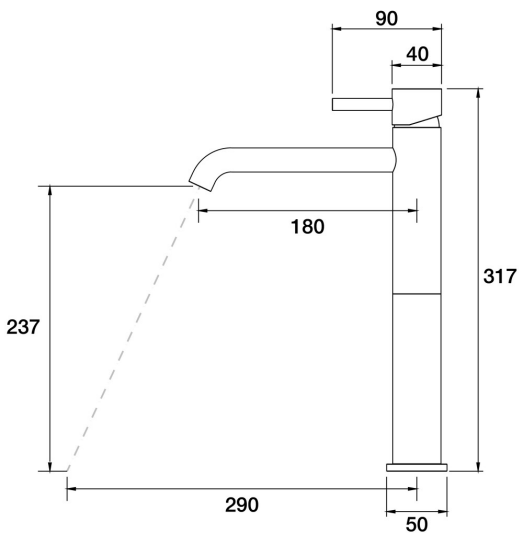
Lugano Hob Basin Tower Mixer A22.012.1.34 - Matt Black
