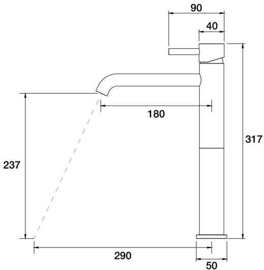
Lugano Hob Basin Tower Mixer A22.012.1.52 - Burnished
