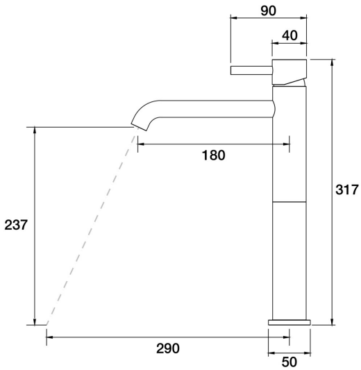
Lugano Hob Basin Tower Mixer A22.012.1.54 - Volcanic Grey
