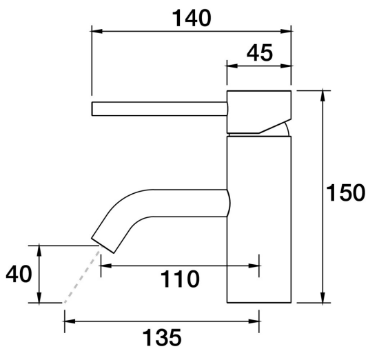
Lugano Hob Basin Mini Mixer DDA Compliant A22.013.2.12 - 23k Brushed Gold
