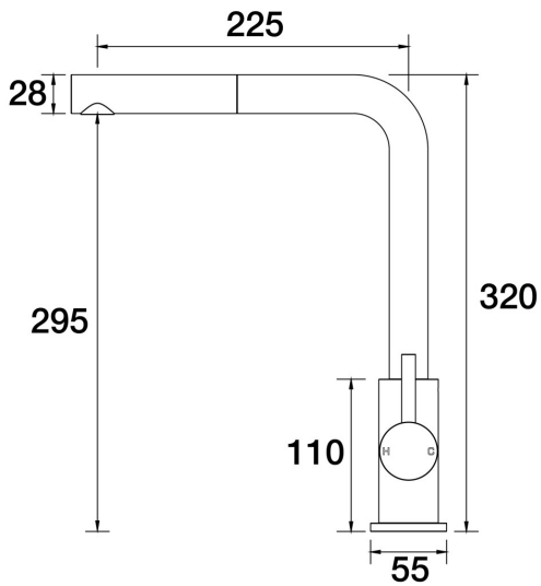
Lugano Sink Straight Mixer Pull-Out - Swivel A22.023.1.42 - Brushed Copper
