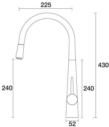
Lugano Sink Pull-Out Mixer A22.024.1.45 - Native Brass
