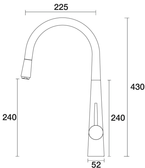
Lugano Sink Pull-Out Mixer A22.024.1.48 - Copper
