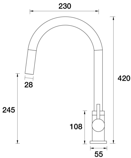
Lugano Sink Pull-Out Mixer Gooseneck A22.024.2.01 - Chrome
