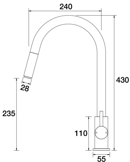
Lugano Sink Pull-Out Mixer Gooseneck A22.024.2.40 - Rumbled Brass
