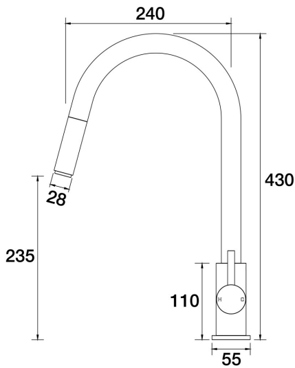
Lugano Sink Pull-Out Mixer Gooseneck A22.024.2.68 - Autumn Bronze
