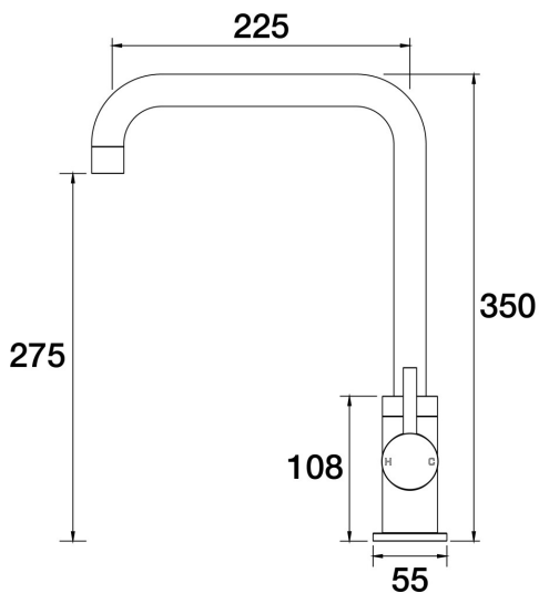
Lugano Sink 90 Degree Mixer A22.025.1.23 - Gunmetal
