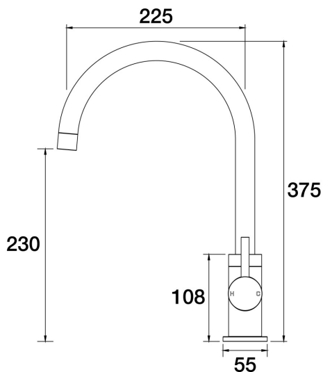
Lugano Sink Gooseneck Mixer A22.026.1.02 - Brushed Chrome
