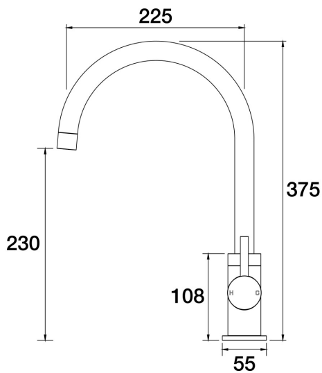
Lugano Sink Gooseneck Mixer A22.026.1.68 - Autumn Bronze
