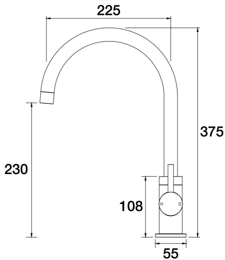
Lugano Sink Gooseneck Mixer A22.026.1.75 - Forest Mist
