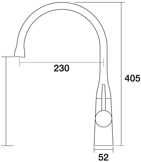
Lugano Sink Gooseneck Mixer Dome A22.026.2.01 - Chrome
