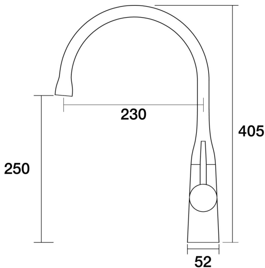
Lugano Sink Gooseneck Mixer Dome A22.026.2.23 - Gunmetal
