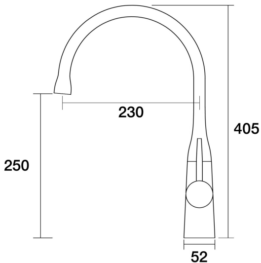
Lugano Sink Gooseneck Mixer Dome A22.026.2.45 - Native Brass
