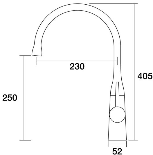
Lugano Sink Gooseneck Mixer Dome A22.026.2.54 - Volcanic Grey
