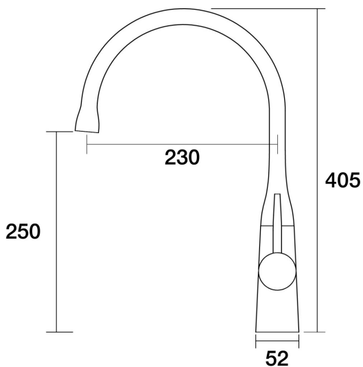
Lugano Sink Gooseneck Mixer Dome A22.026.2.57 - Matt Nickel
