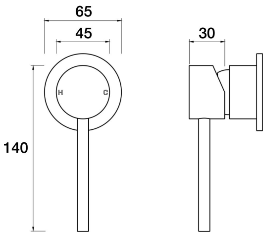
Lugano Wall Mixer Shower DDA Compliant A22.031.2.01 - Chrome
