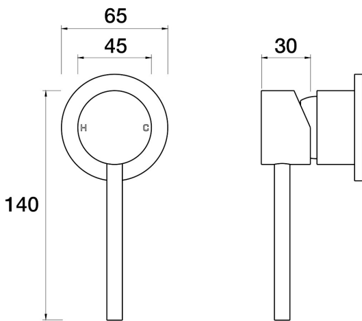
Lugano Wall Mixer Shower DDA Compliant A22.031.2.24 - Brushed Gunmetal
