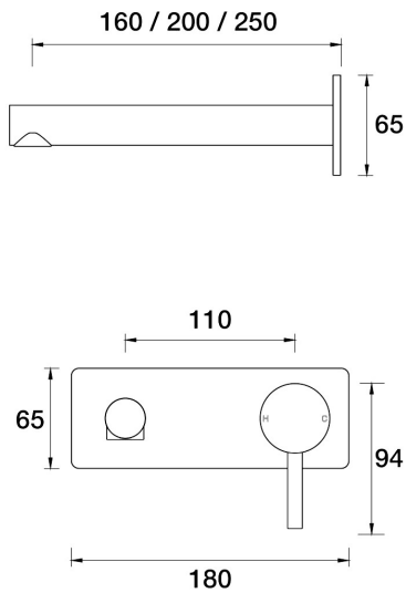
Lugano Wall Mixer Basin Set 200mm outlet Incl. plate A22.032.1.78 - Umber Earth
