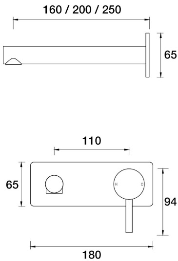
Lugano Wall Mixer Basin Set 250mm outlet Incl. plate
