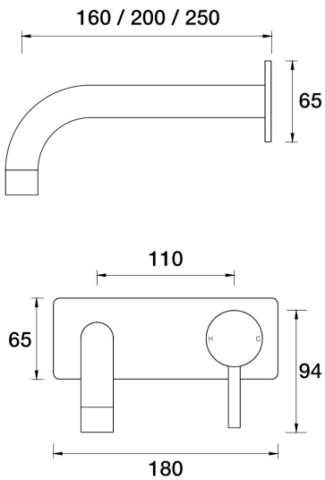
Lugano Wall Mixer Basin Set 200mm 90° outlet Incl. plate A22.032.4.21 - Brushed Rose Gold
