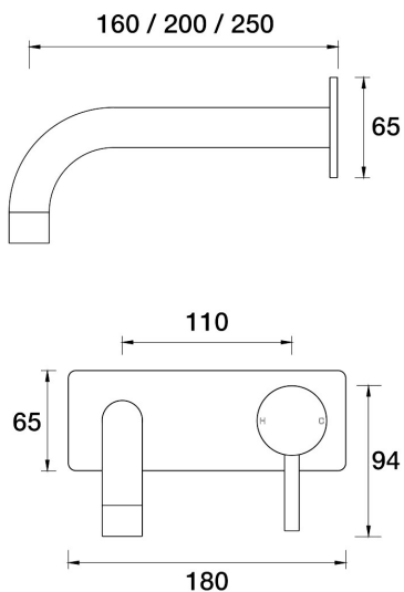
Lugano Wall Mixer Basin Set 160mm 90° outlet Incl. plate A22.032.5.11 - 23k Gold
