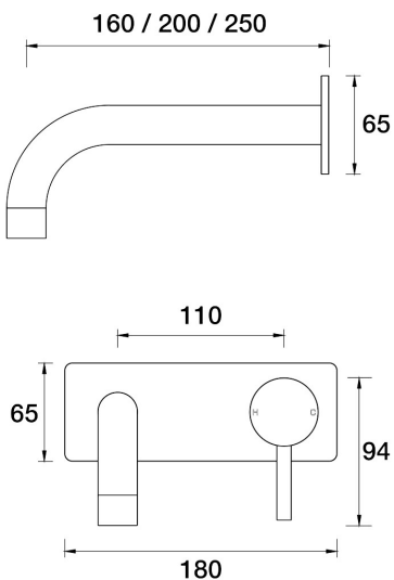
Lugano Wall Mixer Basin Set 250mm 90° outlet Incl. plate A22.032.6.43 - Brass
