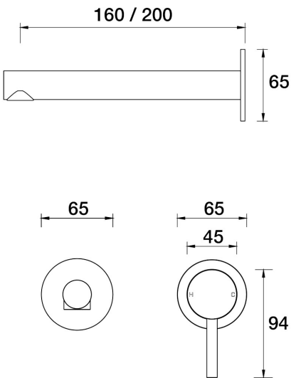
Lugano Wall Mixer Basin Set 200mm outlet A22.033.1.32 - Midnight Black
