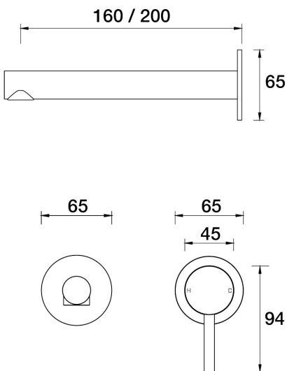
Lugano Wall Mixer Basin Set 200mm outlet A22.033.1.75 - Forest Mist
