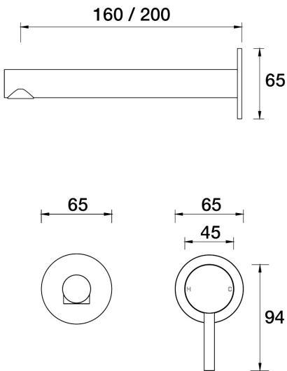
Lugano Wall Mixer Basin Set 160mm outlet A22.033.2.11 - 23k Gold
