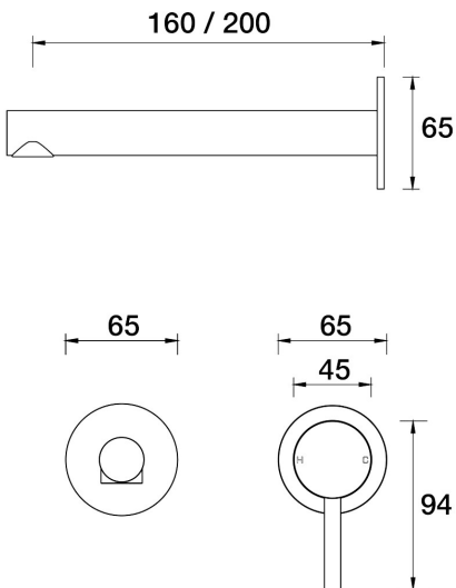
Lugano Wall Mixer Basin Set 160mm outlet A22.033.2.26 - Black Sapphire
