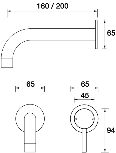
Lugano Wall Mixer Basin Set 200mm 90° outlet A22.033.4.01 - Chrome
