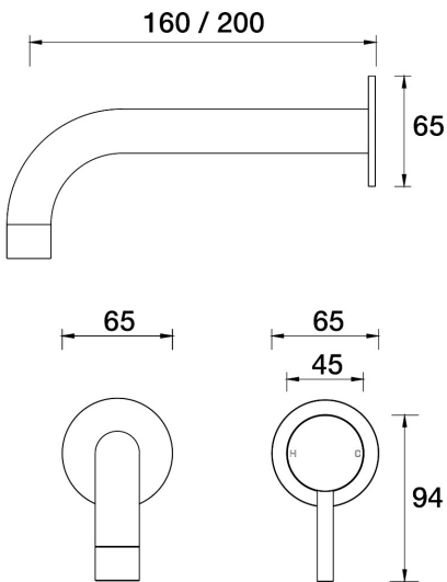
Lugano Wall Mixer Basin Set 200mm 90° outlet A22.033.4.27 - Satin Pearl
