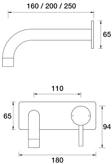
Lugano Wall Bath Mixer Set 250mm 90° outlet Incl. plate A22.041.7.67 - Vintage Brass
