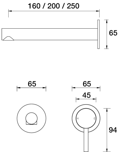
Lugano Wall Bath Mixer Set 160mm outlet A22.043.1.42 - Brushed Copper
