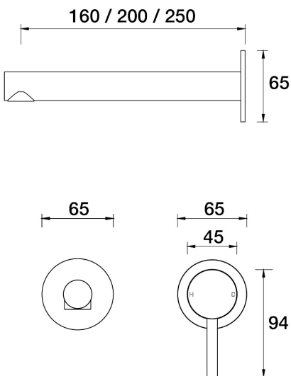
Lugano Wall Bath Mixer Set 200mm outlet A22.043.2.12 - 23k Brushed Gold
