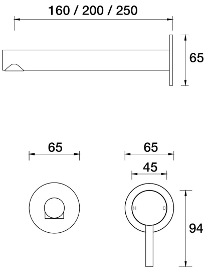
Lugano Wall Bath Mixer Set 200mm outlet A22.043.2.54 - Volcanic Grey
