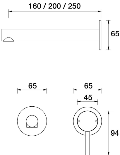
Lugano Wall Bath Mixer Set 200mm outlet A22.043.2.78 - Umber Earth
