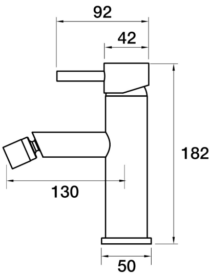
Lugano Bidet Mixer A22.061.1.75 - Forest Mist
