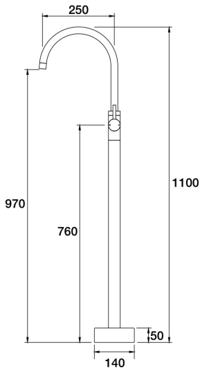
Lugano Floor Bath Filler Mixer - Gooseneck A22.072.1.23 - Gunmetal
