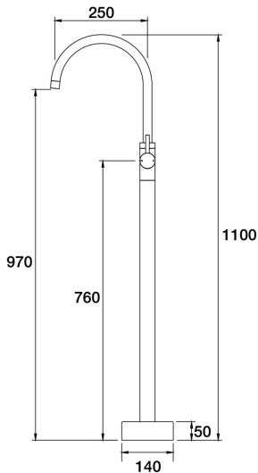
Lugano Floor Bath Filler Mixer - Gooseneck A22.072.1.43 - Brass
