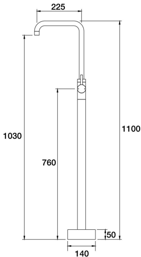
Lugano Floor Bath Filler Mixer - 90 Degree A22.073.1.27 - Satin Pearl
