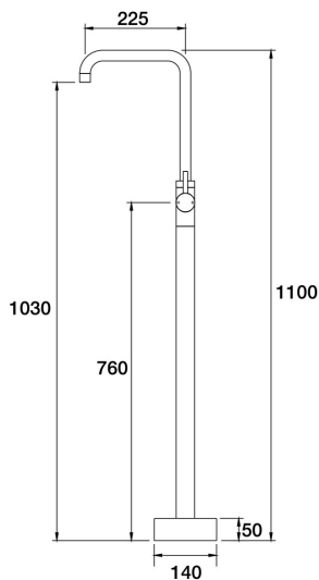
Lugano Floor Bath Filler Mixer - 90 Degree A22.073.1.43 - Brass
