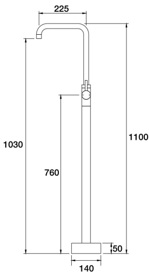
Lugano Floor Bath Filler Mixer - 90 Degree A22.073.1.52 - Burnished
